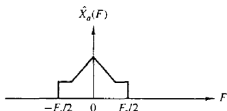
Figure 4.18 Sampling of an analog bandlimited signal and aliasing of spectral components.
